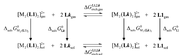
Figure 3. Thermodynamic Born–Haber cycle for ligand exchange reactions of L1 with Lk ( k = 2, 3 ) in the binuclear double-stranded helicates [M_2(L1)_2]^{2+} .
